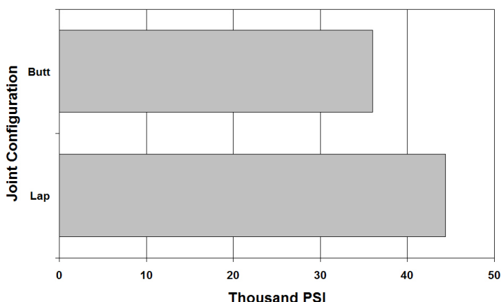
Figure 4: Nicrobraz ® 33 Ultimate Tensile Strength Performance
