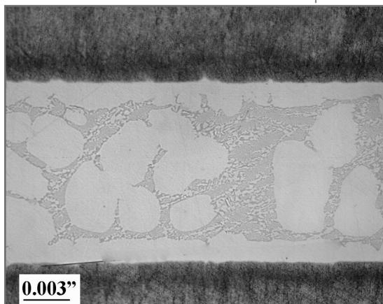
Figure 2: Nicrobraz ® 33 section from variable clearance test showing brazed joint of approximately 0.011" (~0.28mm).
