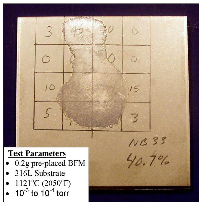
Figure 3: Nicrobraz ® 33 Wetting Test Result
