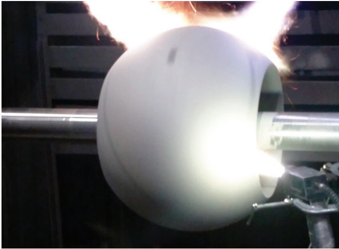
Ball Valve Being Spray & Fused with Wallex® 50 using the J-3 Spraywelder™ System
